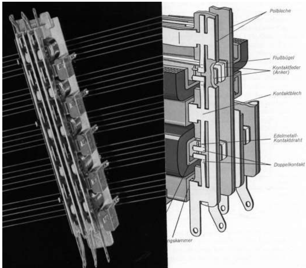
Edelmetall-Schnellrelais
